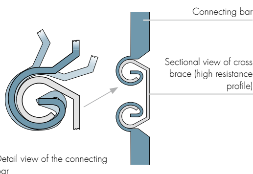
Detail view of the patented safety hinge available for TUBONDA R-type blinds
