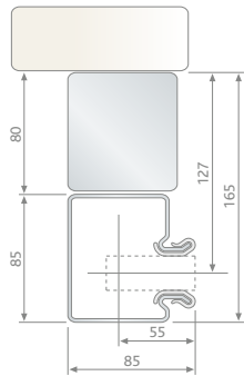
DP 106 guide rails
