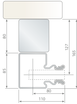
DP 106 guide rails for enhanced wind resistance
