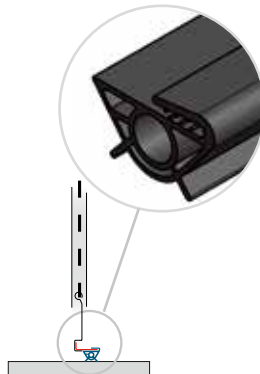
Finishing profile with seal
